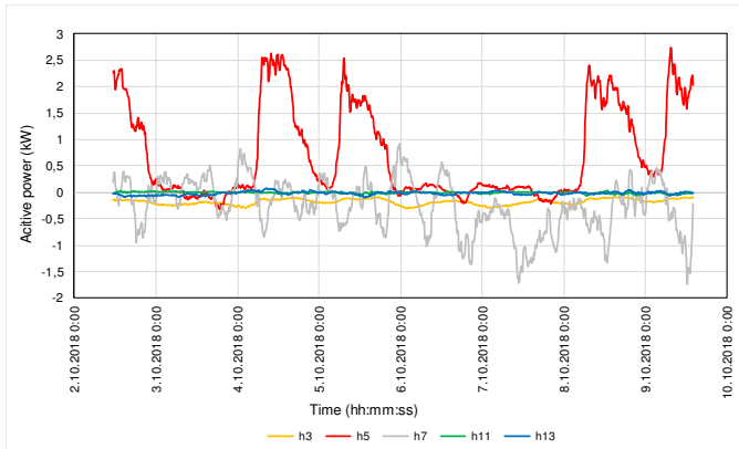
Fig. 11. Calculated power for relevant harmonics
